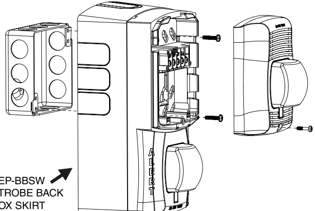
SEP-SW for surface-mount applications
